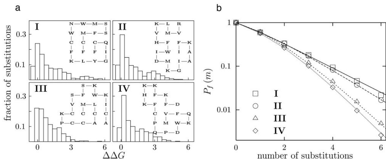
Fig. 1. Lattice proteins with different structures but the same stability ( \Delta G_f = -1.0 ) converge to different exponential declines in m -neutrality. (a) The distributions of \Delta\Delta G for all 380 single amino acid substitutions to the inset lattice proteins. (b) The measured (symbols) and predicted (lines) m -neutralities for the four proteins. Proteins are considered folded if \Delta G_f \leq 0.0 for the original native structure. The proteins used for the m -neutrality analyses were generated by adaptive walks from random starting sequences, followed by 2.5 \times 10^5 generations of neutral evolution with a population size of 100 and a per-generation per-residue substitution rate of 5 \times 10^{-5} , selecting for sequences with \Delta G_f \leq -1.0 and then taking the first sequence generated with a stability within 0.025 of -1.0 . The m -neutralities were computed by sampling all mutants for m \leq 2 or 5 \times 10^3 random mutants for m > 2 . The predicted m -neutralities were computed according to Eq. 1 by numerically convolving the distribution of single-substitution \Delta\Delta G values using generating functions (27) computed with fast-Fourier transforms and a bin size of 0.01.
